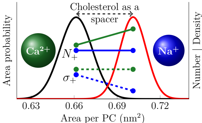
Figure 4: Schematic picture describing the effect of cholesterol on cation adsorption. Black and red curves show the distribution of the area per phospholipid in POPC membranes with 0% and 30% cholesterol, respectively. Green and blue lines show data for the effect of cholesterol-induced area increase on calcium and sodium adsorption respectively; solid lines show the number of adsorbed ions ( N_+ ), while the dashed lines show the resulting surface charge density ( \sigma_+ ). The number of bound calcium ions is proportional to the total area, resulting in a constant surface charge density. The number of sodium ions, on the other hand, is proportional to the number of PC head groups, resulting in a surface charge density that is proportional to the area per PC lipid. Note that this figure depicts trends, whereas the data is properly shown in Figs. 2 and 3.
