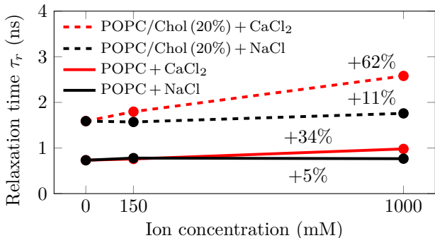
Figure 1: Relaxation times from time-dependent fluorescence shift measurements at 310 K. The percentage values represent the relative increase of Laurdan relaxation times upon the addition of 1 M of salt. Whereas the methodology itself is quite precise (error of \sim 0.05 ns), we estimate the total error associated with the values for the relative increase to be \sim 10 percentage points, estimated from comparing values obtained using different fitting strategies.
