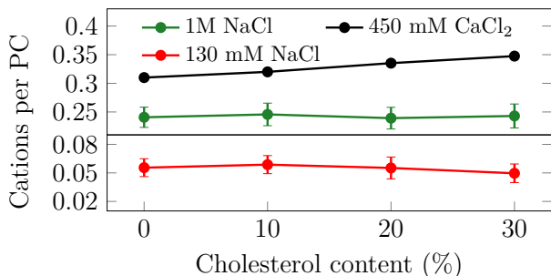
Figure 2: Average number of bound cations per POPC head group as a function of cholesterol concentration. Error bars show Std. Dev.
