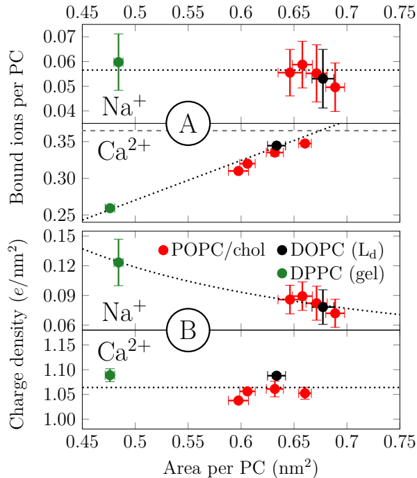
Figure 3: (A) The dependence of cation adsorption (130 mM of NaCl or 450 mM of CaCl 2 ) on the area per PC. (B) The dependence of surface charge density on the area per PC in membranes. Red dots are POPC with 0, 10, 20, or 30% cholesterol at 310 K (smallest to highest area). Black dot is DOPC at 310 K. Green dot is DPPC at 295 K. Dashed lines show fits to the data, see text for details. Error bars show Std. Dev.
